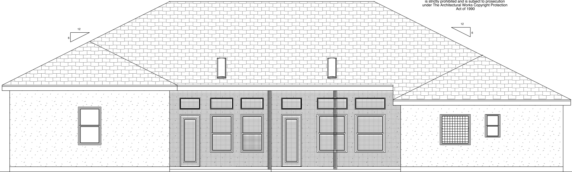
Rear Elevation
